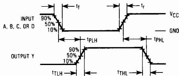
Figure 1. Switching Waveforms
