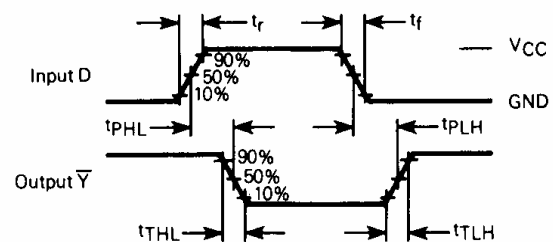
Figure 2. Switching Waveforms
