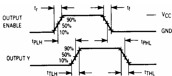
Figure 3. Switching Waveforms
