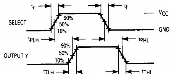
Figure 2. Switching Waveforms
