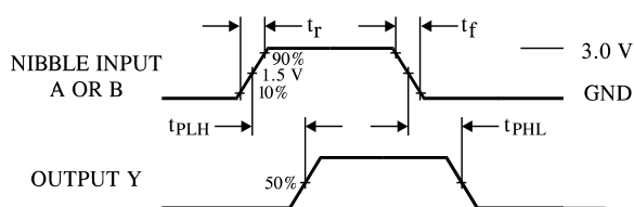
Figure 1. Switching Waveforms
