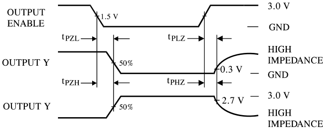
Figure 3. Switching Waveforms
