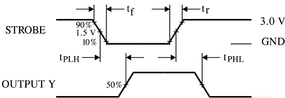
Figure 4. Switching Waveforms
