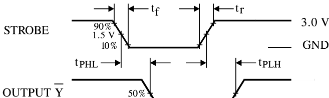
Figure 5. Switching Waveforms
